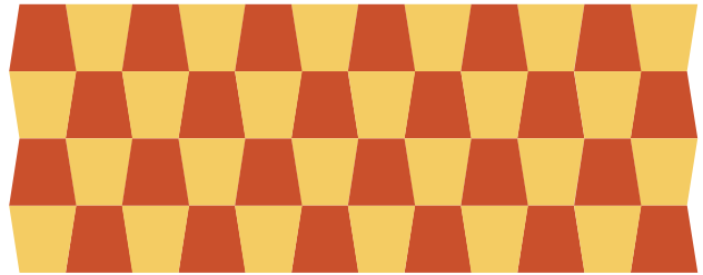
Figure 1.1: A tessellation of isosceles trapezoids
